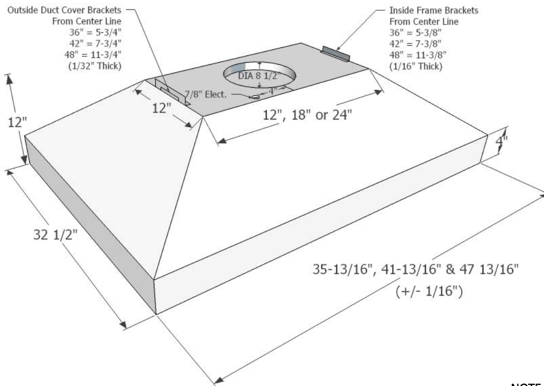
Wood Mounting Frame & Duct Cover
