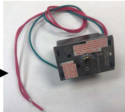
CURRENT CSWITCH170—5 AMP 2 MOTORS GREEN GROUND WIRE
